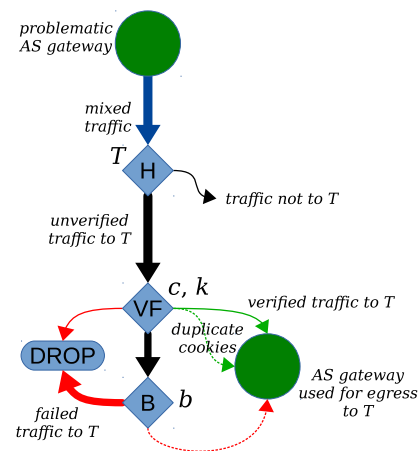
Fig. 2. Separation of verified traffic from unverified in a single AS
