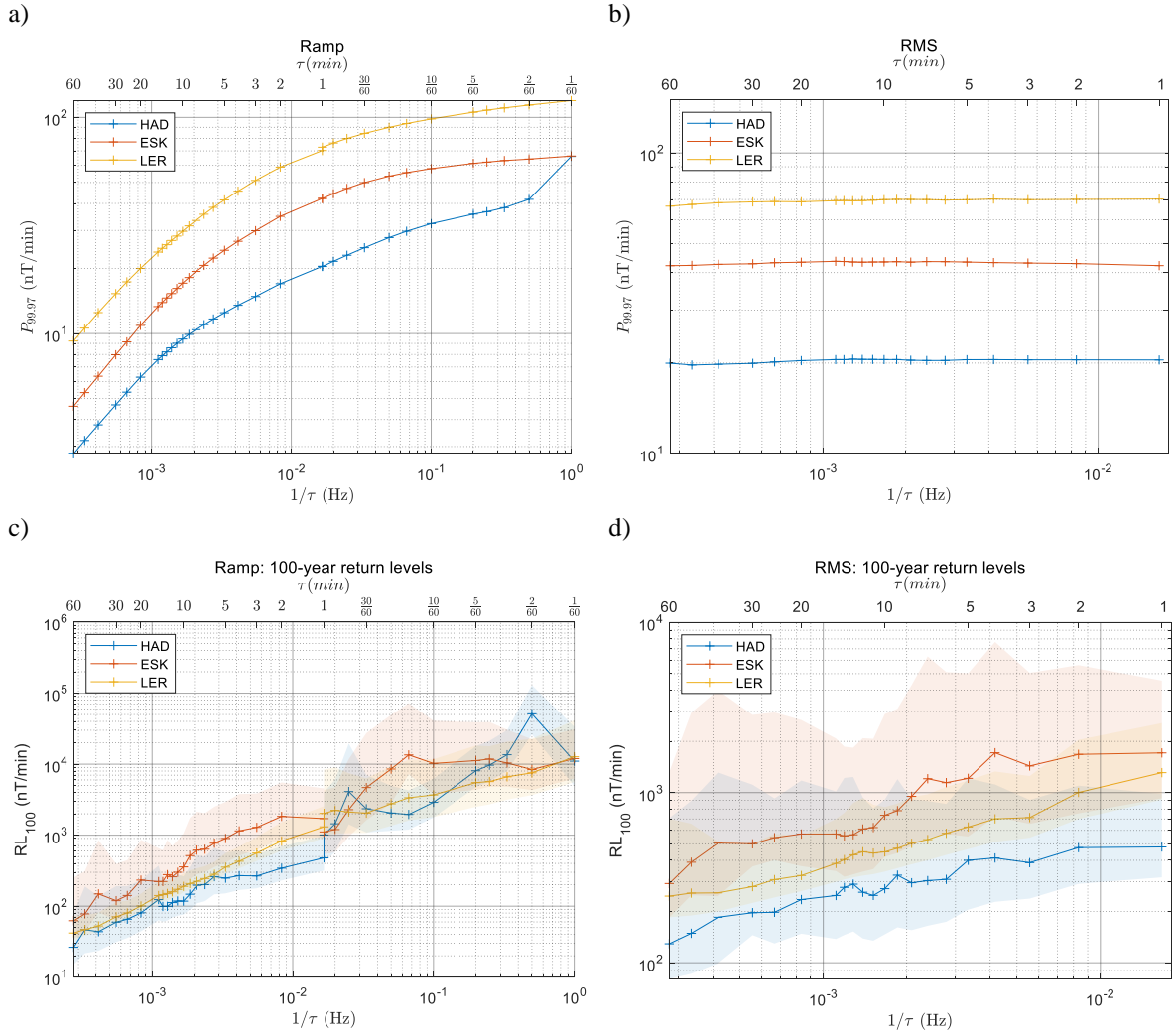
Figure 14. a) P_{99.97} of R_n , b) P_{99.97} of S_n , c) 100-year RLs of R_n , and d) 100-year RL of S_n , for three UK sites. RLs are maximum likelihood estimates, whilst the shaded regions indicate 95% confidence intervals.
