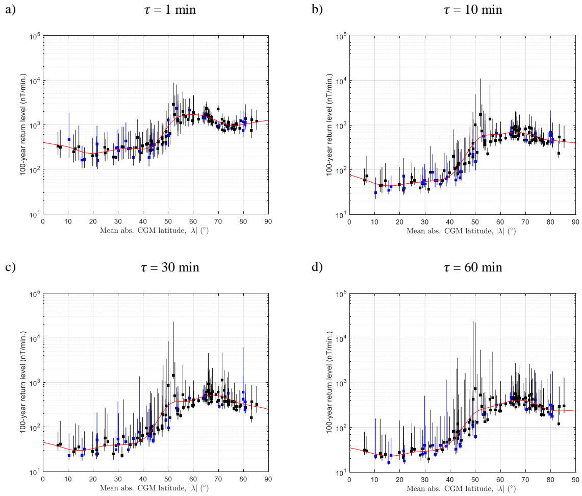
Figure 9. 100-year return levels (Max. likelihood estimates with 95% CI shown as error bars) for RMS variations ( \mathcal{S}_n ). Black indicates NH sites, blue indicates SH. a) \tau = 1 min, b) \tau = 10 min, c) \tau = 30 min, and d) \tau = 60 min. The red curves are smoothed spline fits to MLEs.
