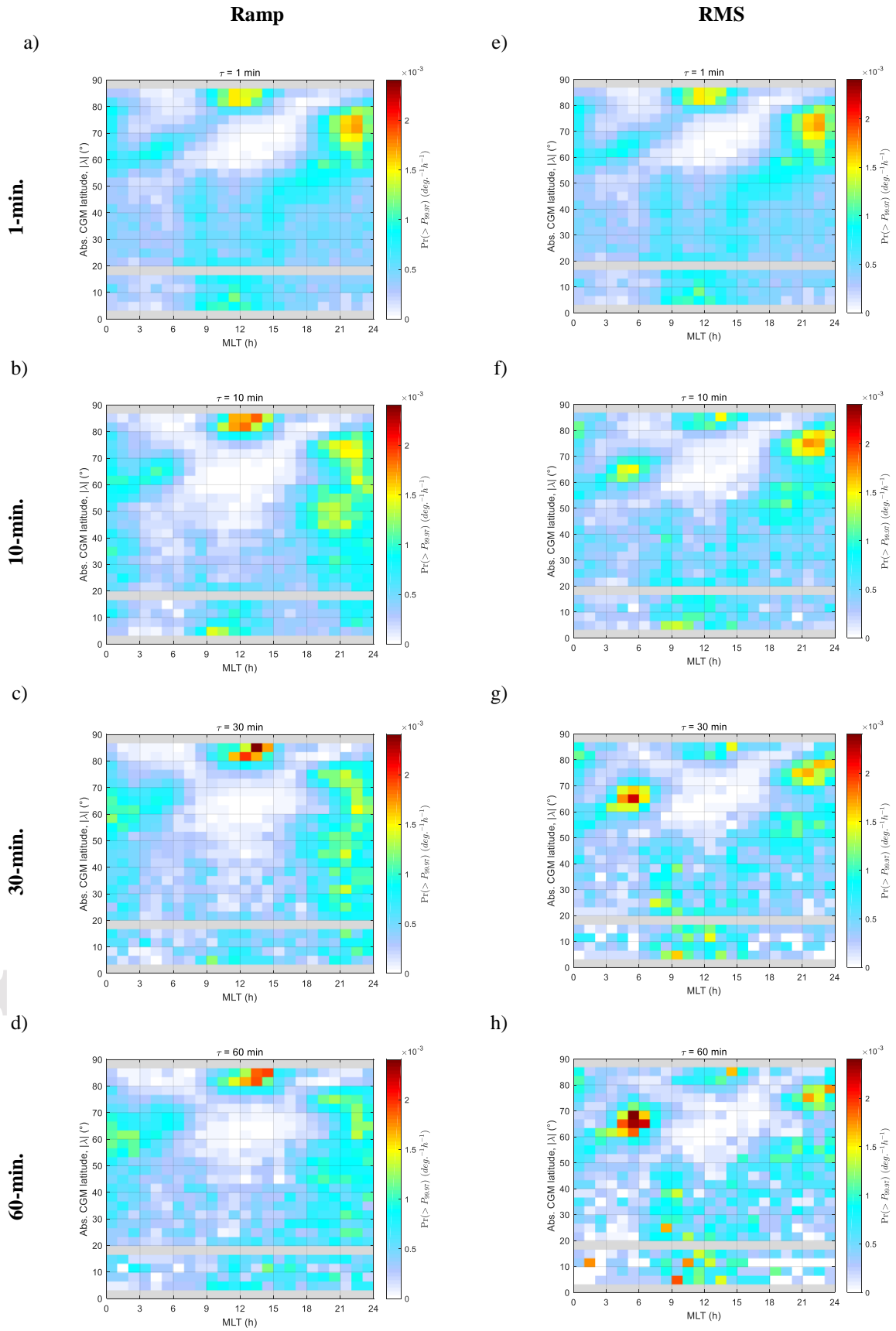
Figure 2. \Pr(|dB_h/dt| > P_{99.97}) against CG latitude and MLT for (a) R_1 , (b) R_{10} , (c) R_{30} , (d) R_{60} , (e) S_1 ( = R_1 ), (f) S_{10} , (g) S_{30} , (h) S_{60} . Latitude bins with no magnetometers are coloured grey.
