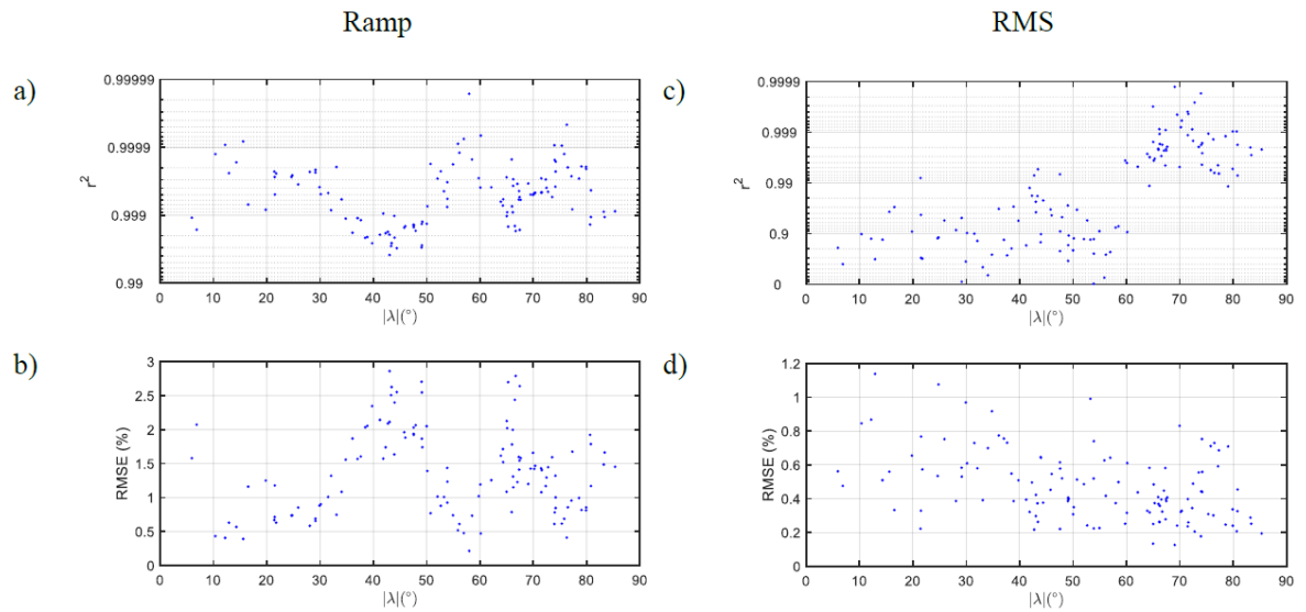
Figure 6. Goodness-of-fit metrics for the polynomial fit to \log P_{99.97}(\log f_s) for (a, b) Ramp changes, and (c, d) RMS variations. Top panels (a, c) are coefficients of determination, r^2 . Bottom panels (b, d) are the RMS of residuals.
