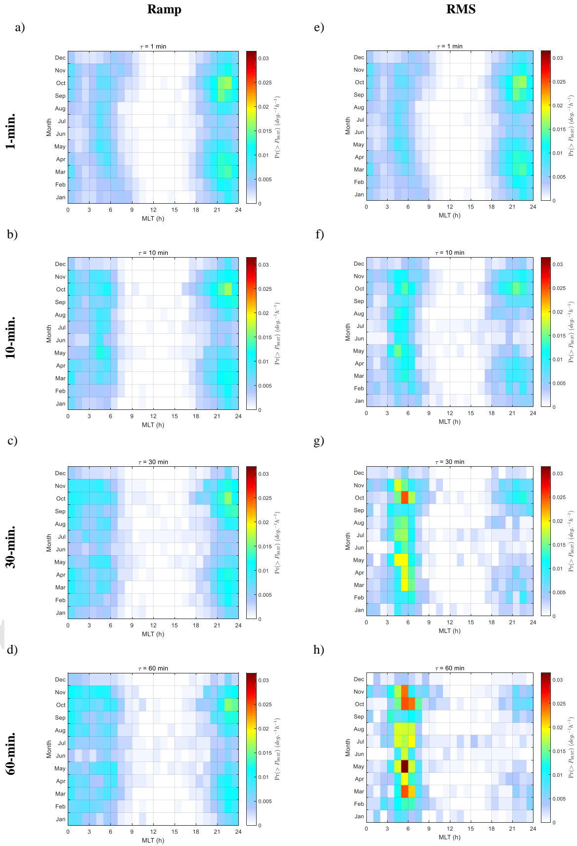
Figure 3. Pr(|dB_h/dt| > P_{99,97}) vs (MLT, month) for (a) R_1 , (b) R_{10} , (c) R_{30} , (d) R_{60} , (e) S_1 (= R_1) , (f) S_{10} , (g) S_{30} , (h) S_{60} for stations between 60 – 70°N CG latitude.
